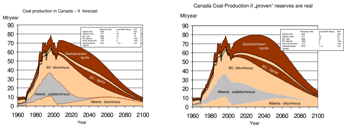
Figure A-13: Production forecast “low” and “high”
