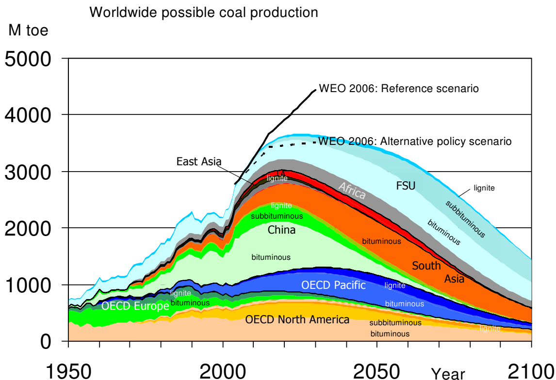
Figure 5: World coal production in the equivalent of a million tons of oil as calculated in this study based on proved recoverable reserves.
